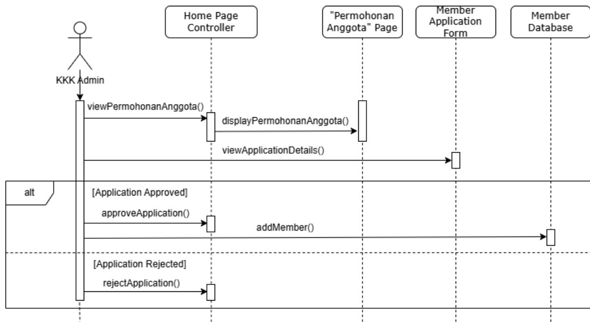
Figure 4.25: SD008 Sequence Diagram for Approve Membership
