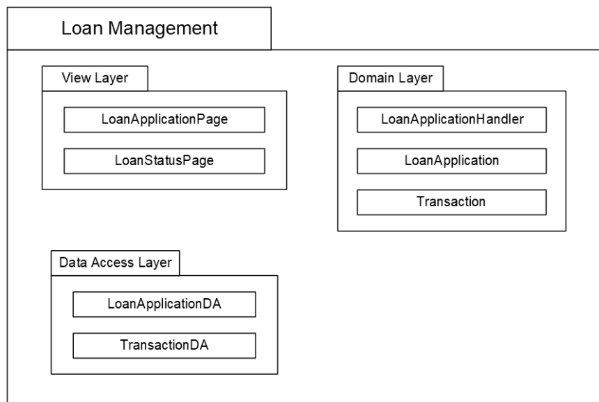
Figure 4.7 Package Diagram for Loan Management Subsystem
