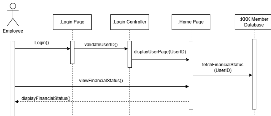
Figure 4.19: SD002 Sequence Diagram for Log In
