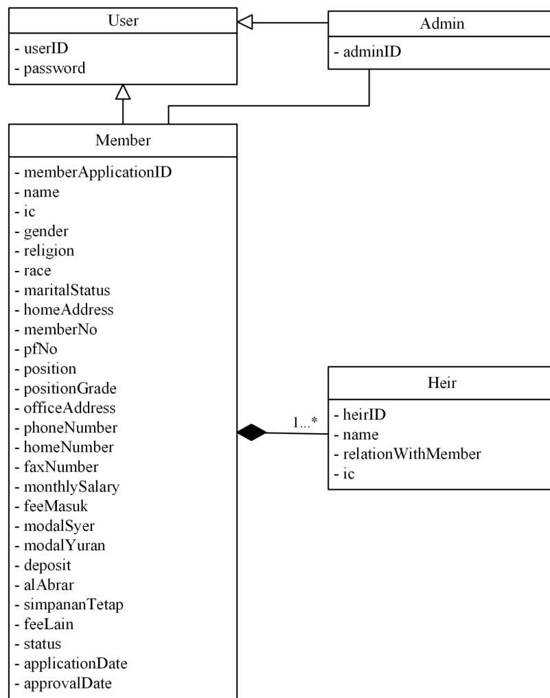
Figure 4.12 Class Diagram for User Module
