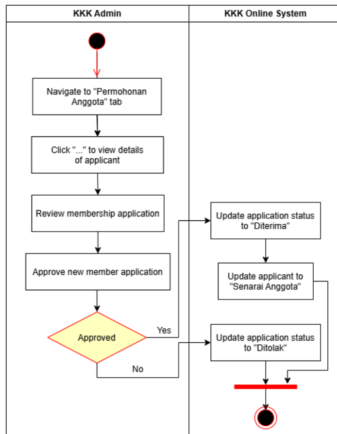
Figure 2.20: Activity Diagram for Approve New Member Application
