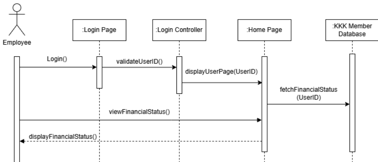
Figure 4.21: SD004 Sequence Diagram for View Financial Status
