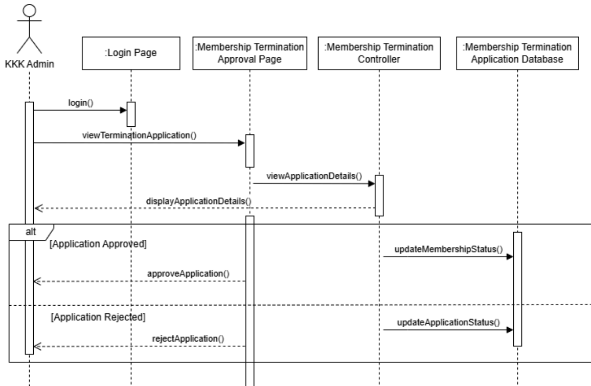
Figure 2.27: Sequence Diagram for Approve Member Termination
