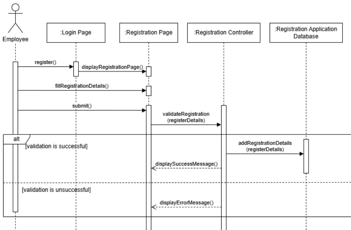
Figure 2.5: Sequence Diagram for Apply Membership
