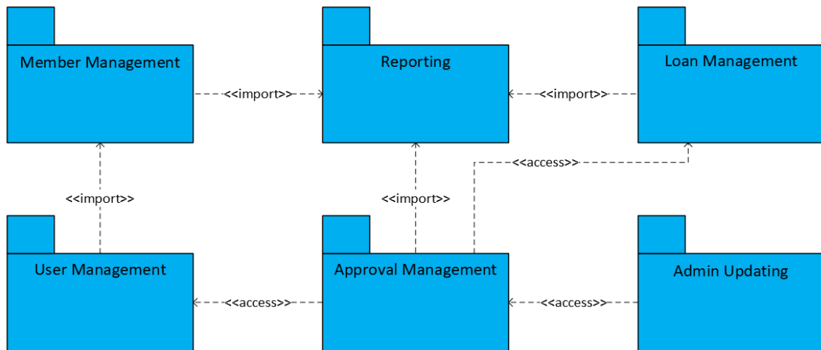
Figure 4.4 Package Diagram for KKK Online System
