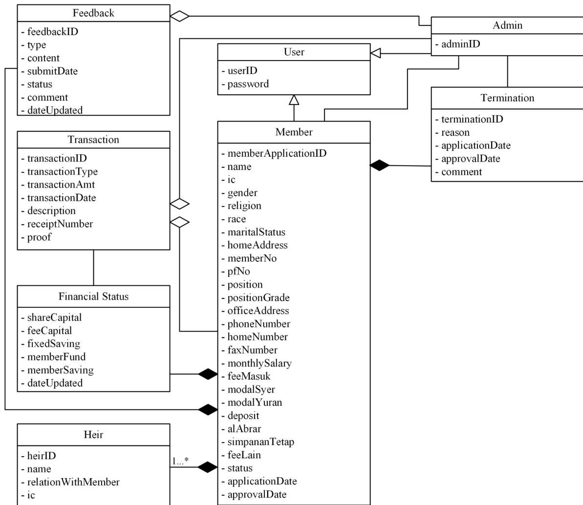
Figure 4.13 Class Diagram for Member Module
