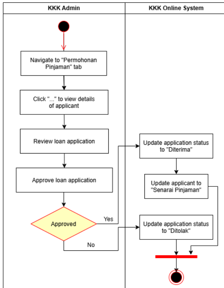
Figure 2.22: Activity Diagram for Approve Loan Application
