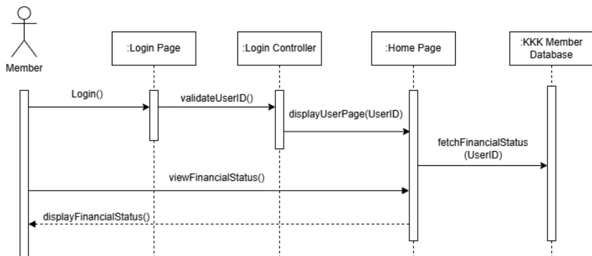
Figure 2.11: Sequence Diagram for View Financial Status
