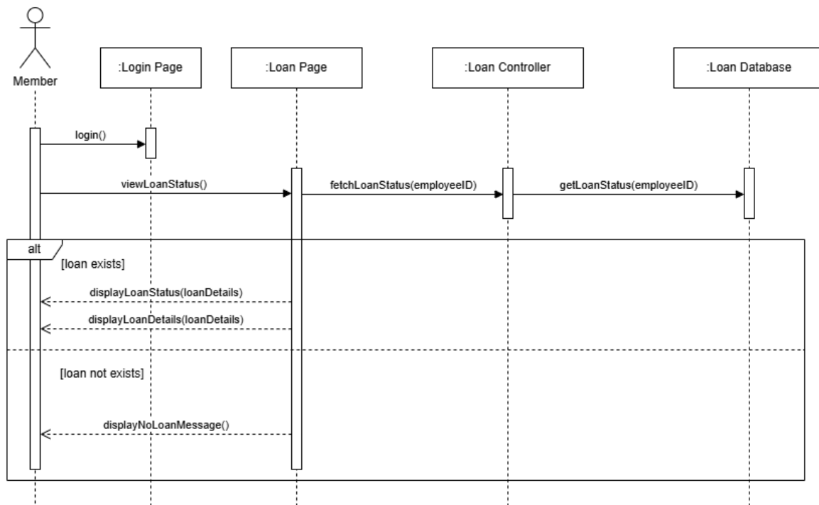
Figure 4.23: SD006 Sequence Diagram for View Loan Application Status
