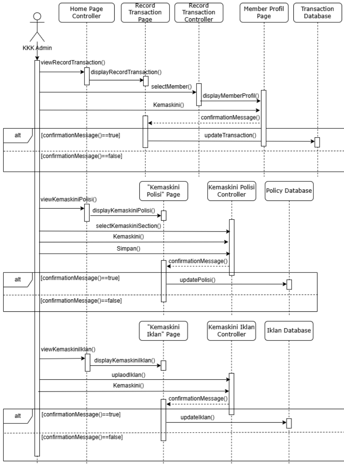
Figure 4.28: SD011 Sequence Diagram for Administer
