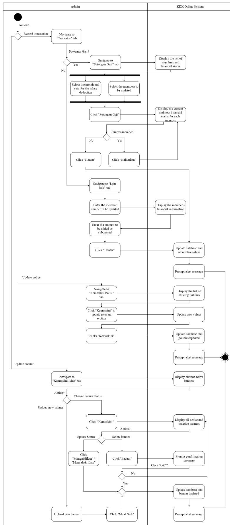
Figure 2.26: Activity Diagram for Manage System
