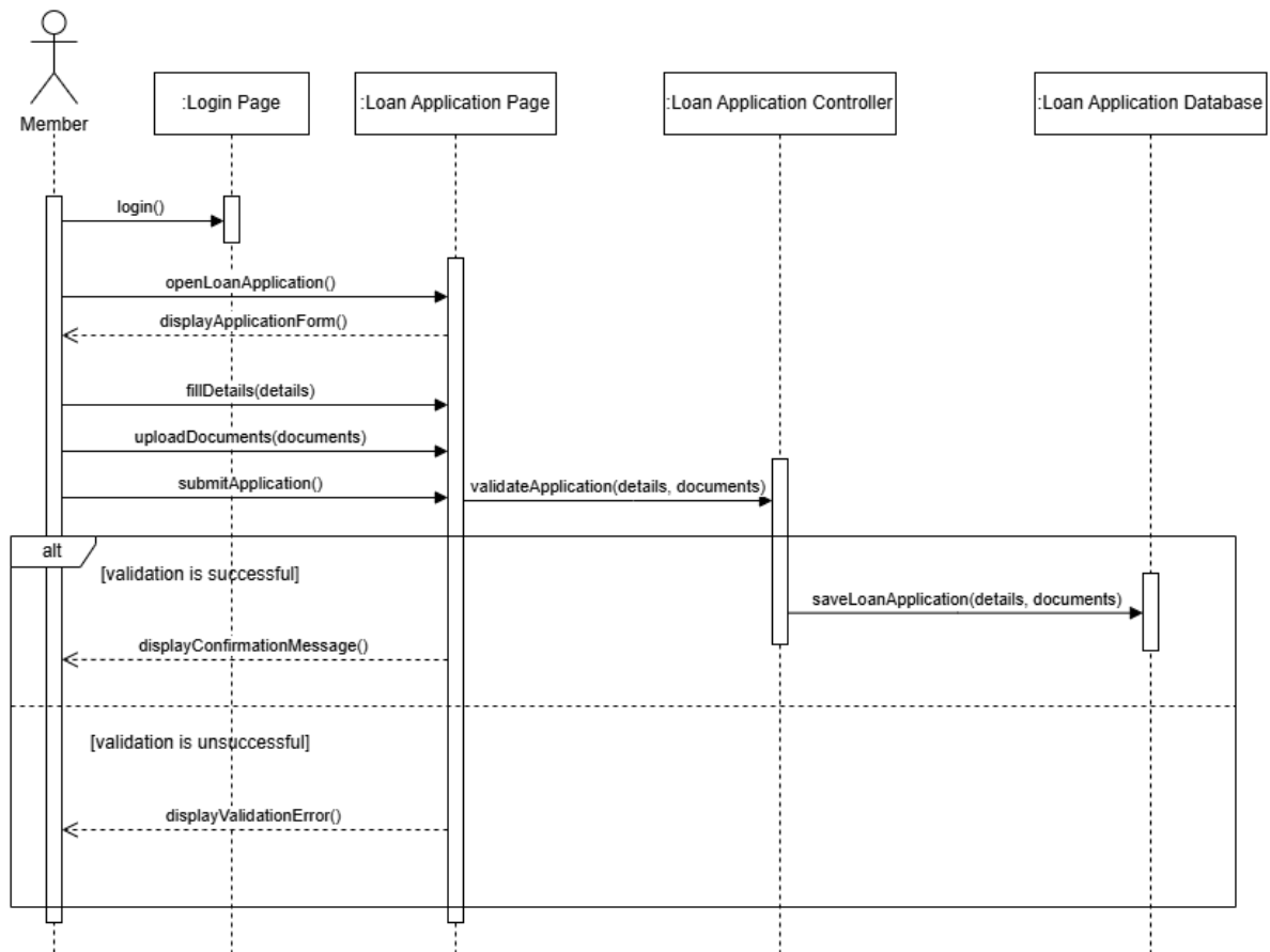
Figure 4.22: SD005 Sequence Diagram for Apply Loan
