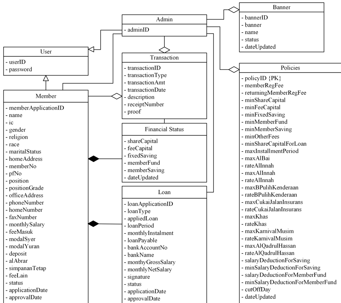
Figure 4.16 Class Diagram for Admin Updating Module
