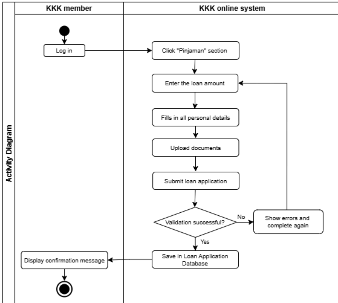
Figure 2.14: Activity Diagram for Apply for a loan
