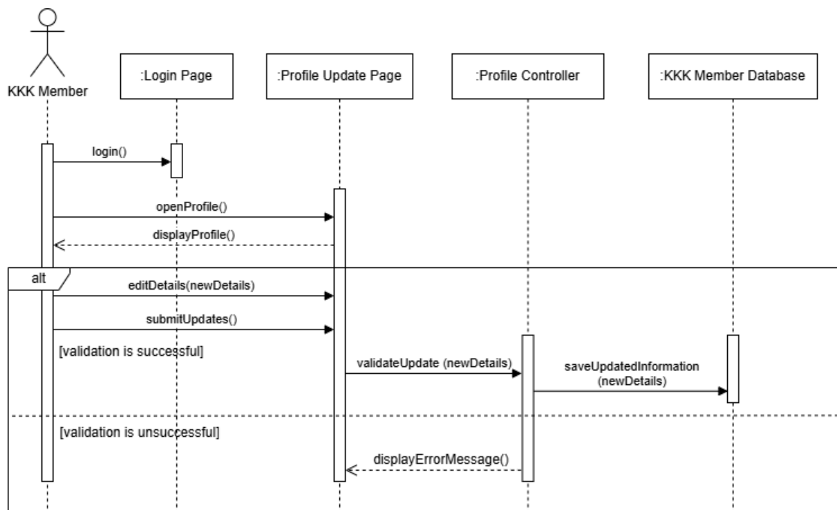
Figure 2.7: Sequence Diagram for Update User Profile
