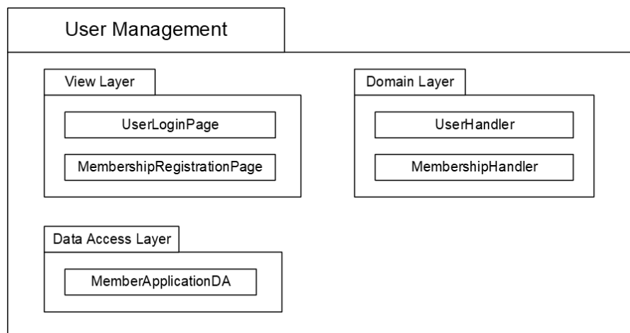
Figure 4.5 Package Diagram for User Management Subsystem
