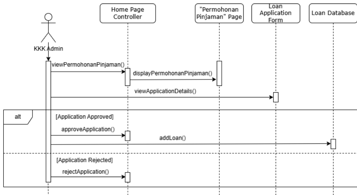
Figure 2.21: Sequence Diagram for Approve Loan Application
