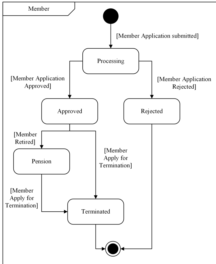
Figure 2.3: State Machine Diagram for Member Class
