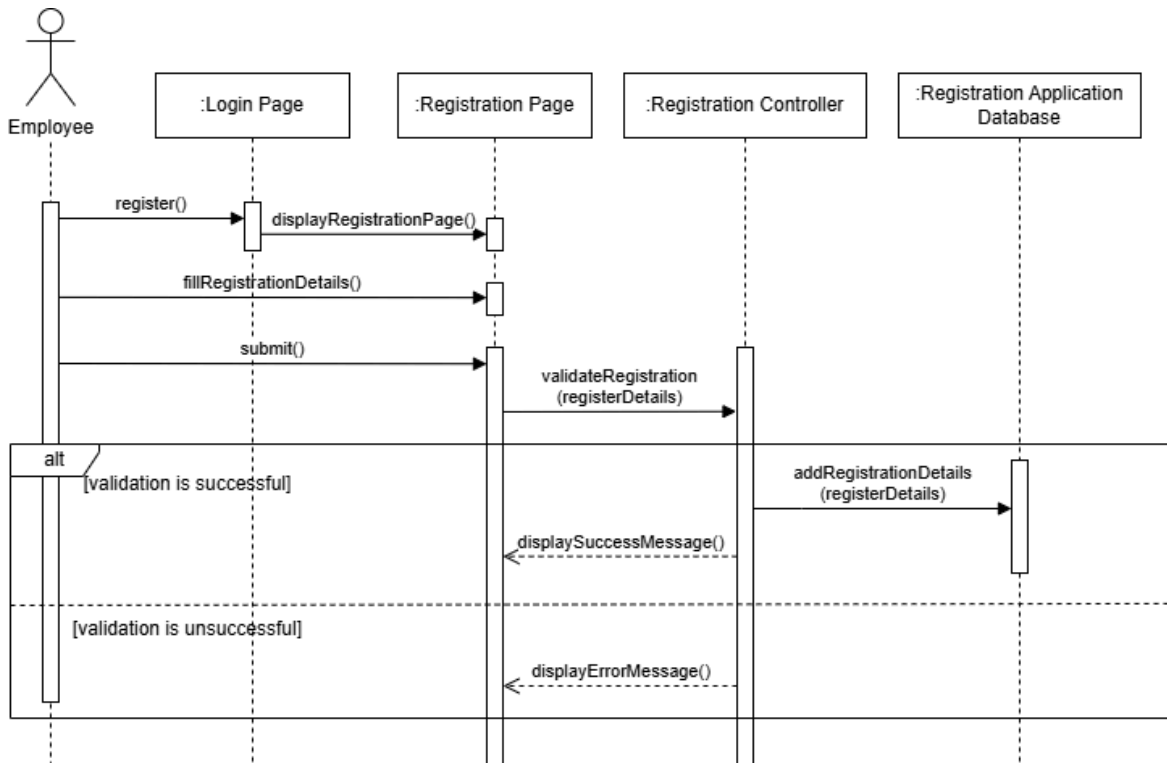
Figure 4.18: SD001 Sequence Diagram for Apply Membership
