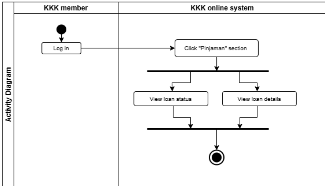
Figure 2.16: Activity Diagram for View Loan Application Status
