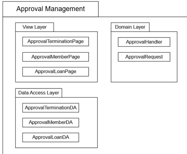
Figure 4.8 Package Diagram for Approval Management Subsystem
