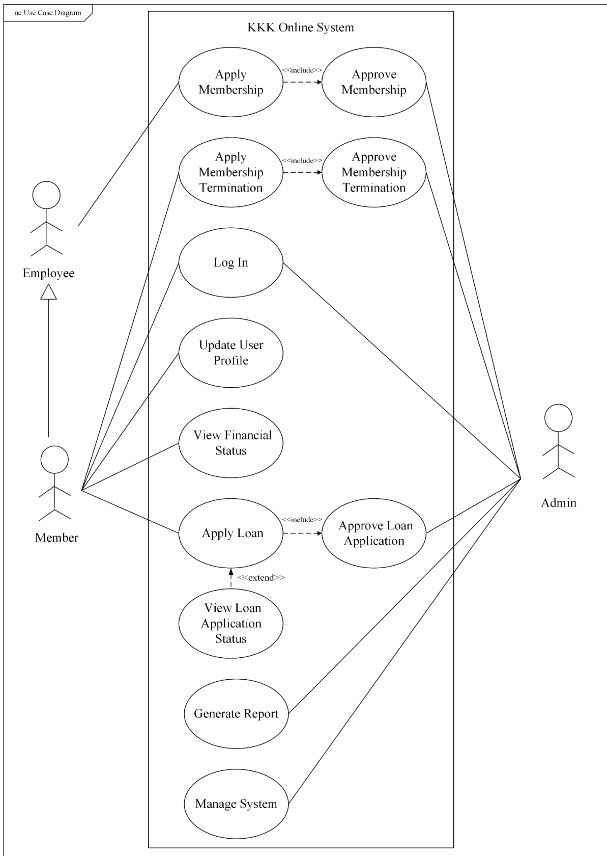
Figure 4.2 Use Case Diagram for KKK Online System
