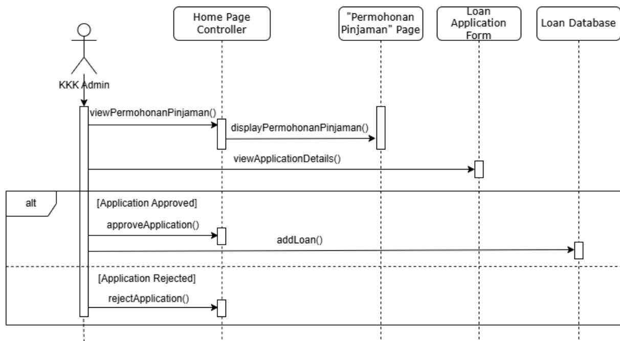
Figure 4.26: SD009 Sequence Diagram for Approve Loan Application
