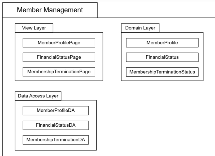
Figure 4.6 Package Diagram for Member Management Subsystem
