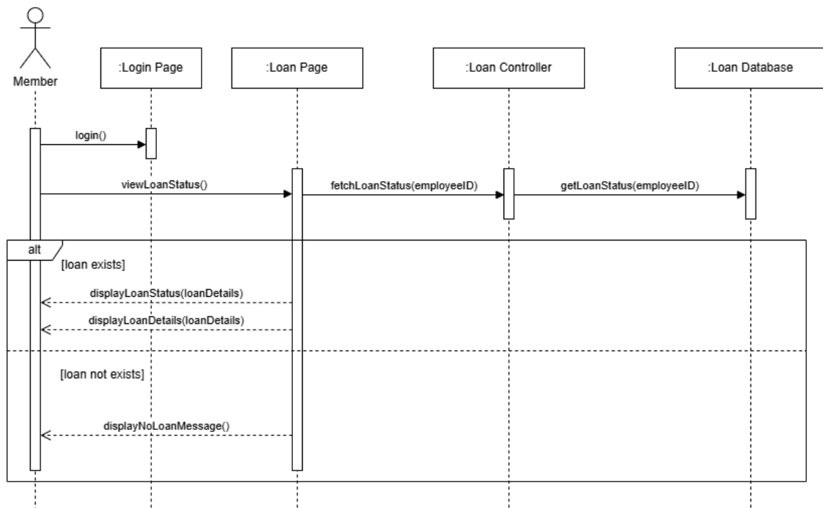
Figure 2.15: Sequence Diagram for View Loan Application Status
