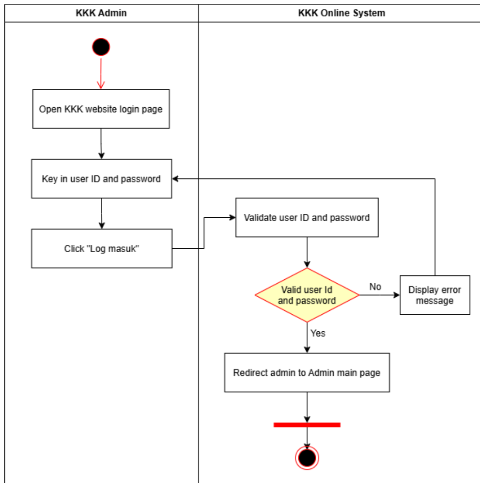
Figure 2.10: Activity Diagram for Login
