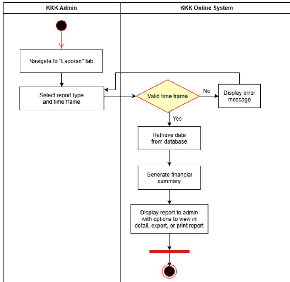
Figure 2.24: Activity Diagram for Generate Report
