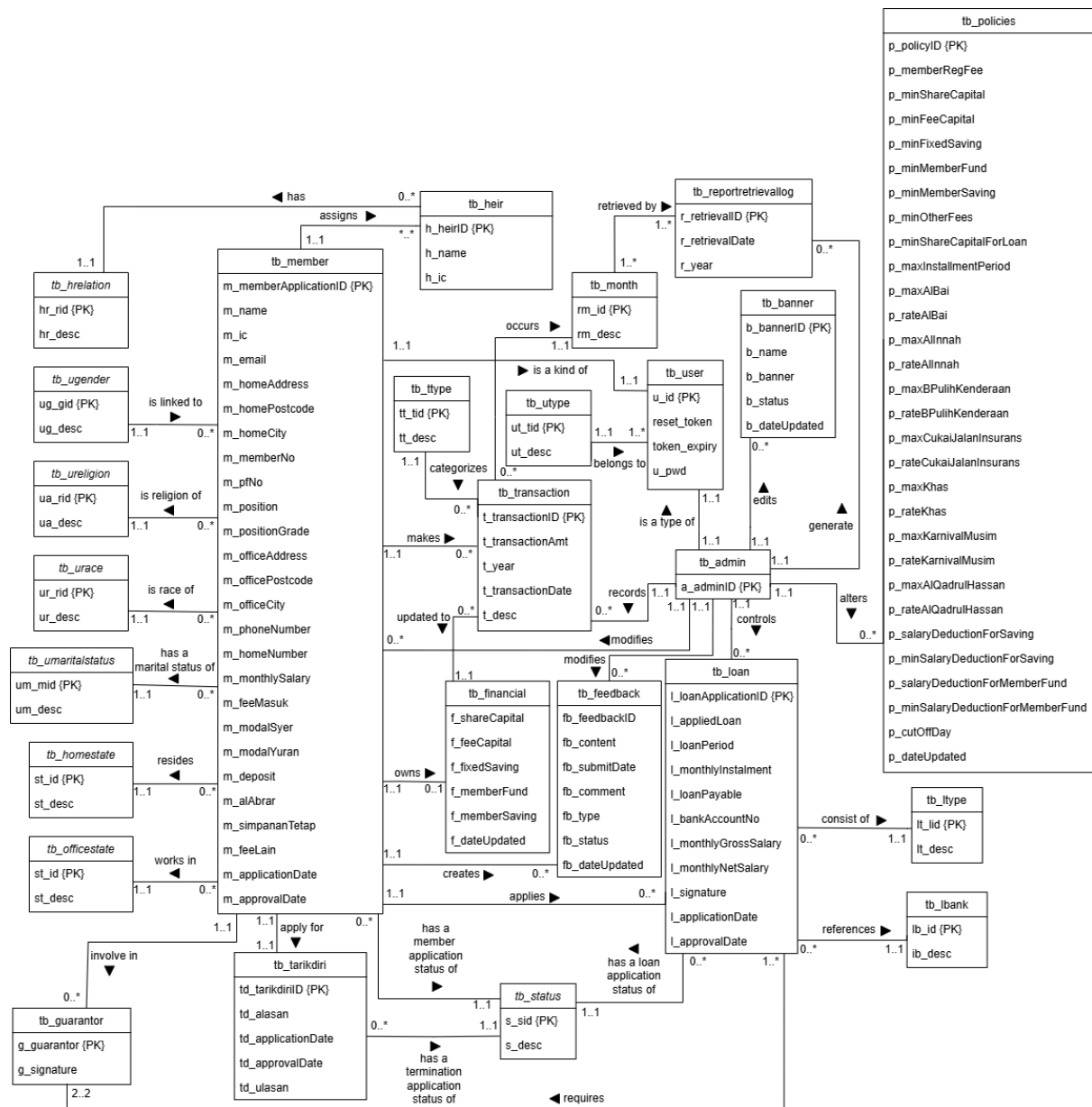
Figure 5.1 Entity-Relationship Diagram For KKK System
