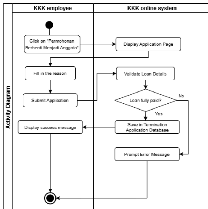
Figure 2.18: Activity Diagram for Apply Membership Termination
