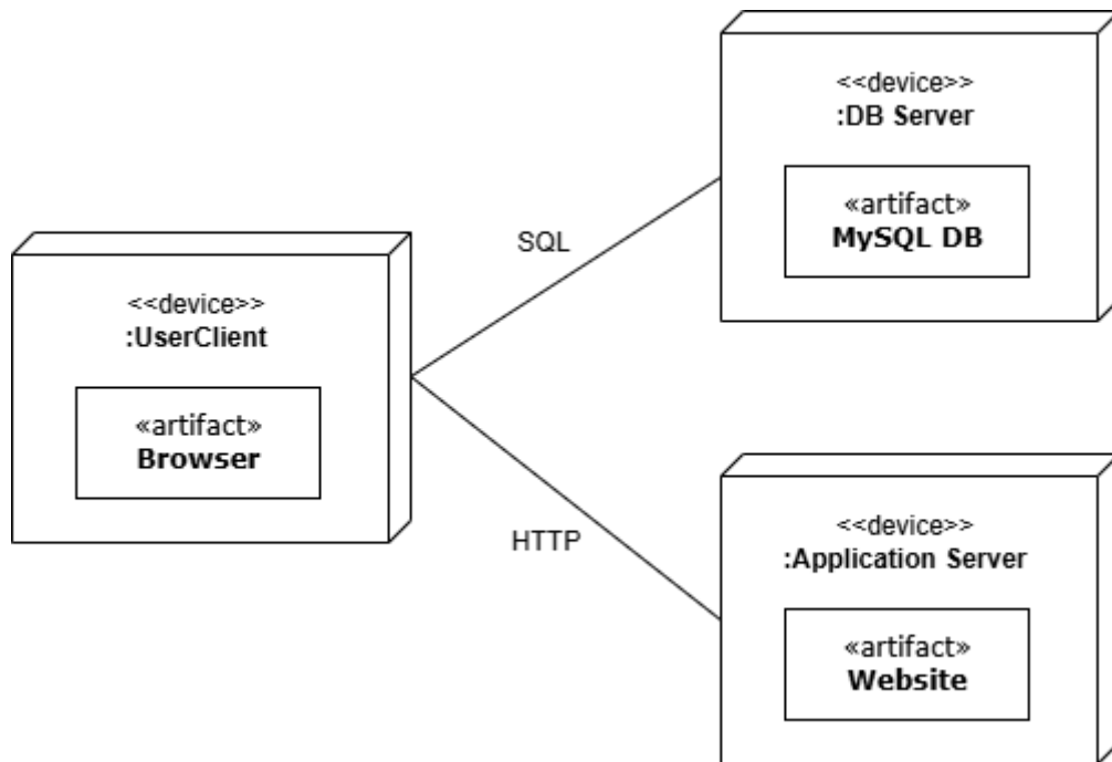
Figure 4.29: Deployment diagram for KKK Online System
