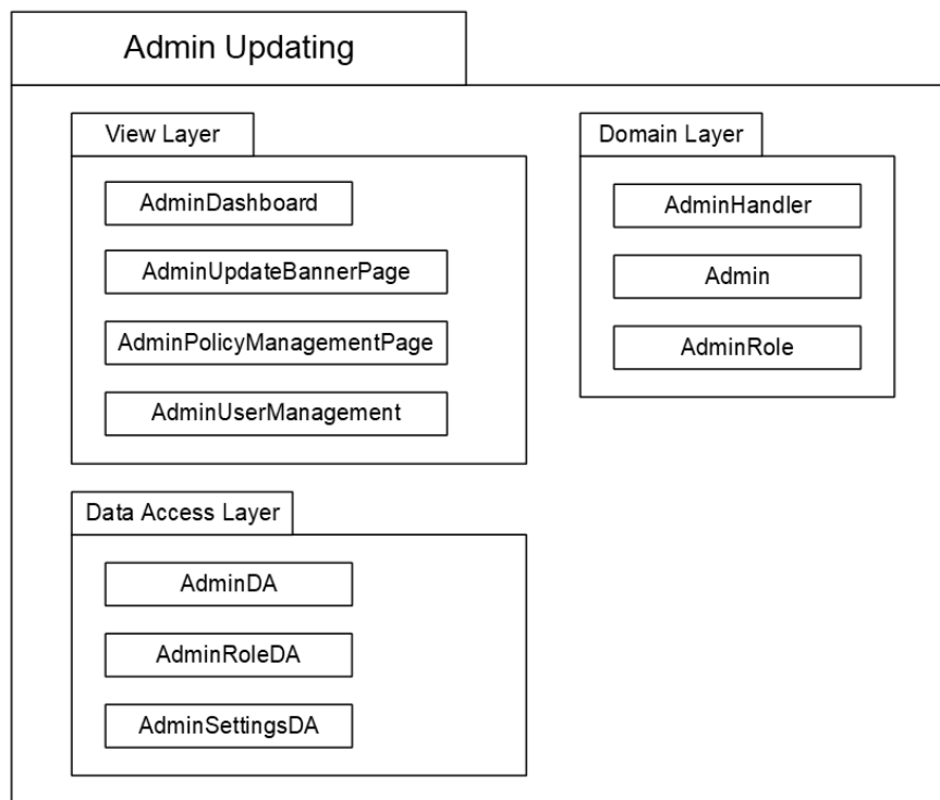
Figure 4.9 Package Diagram for Admin Updating Subsystem
