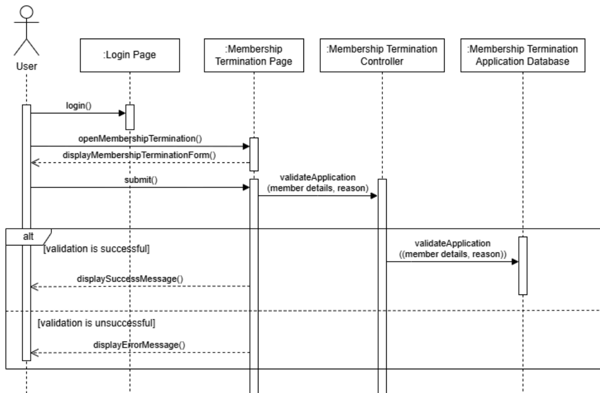
Figure 2.17: Sequence Diagram for Apply Membership Termination
