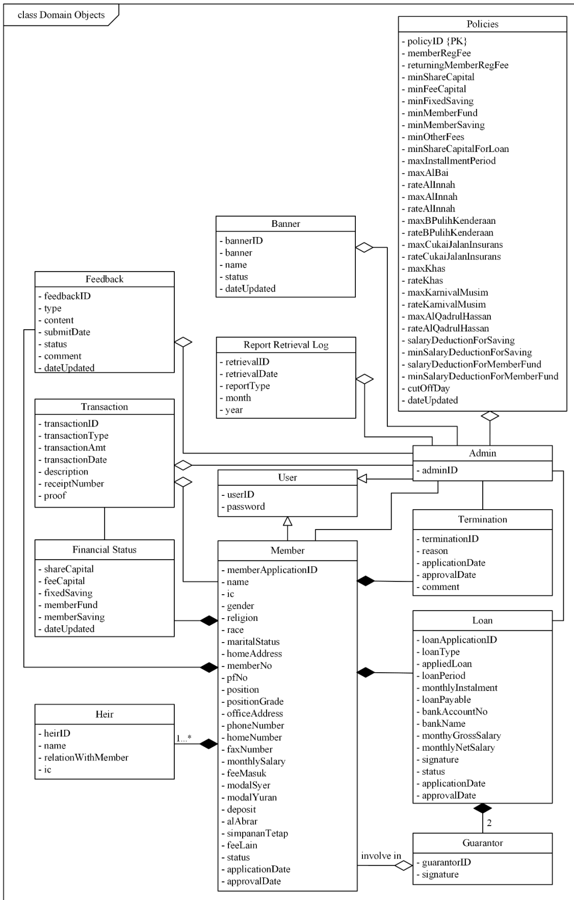
Figure 4.11 Class diagram for KKK Online System
