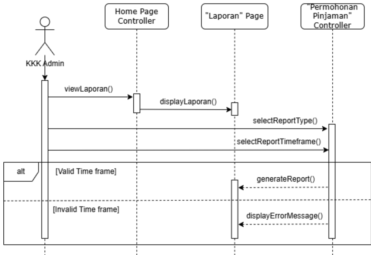
Figure 4.27: SD010 Sequence Diagram for Generate Report
