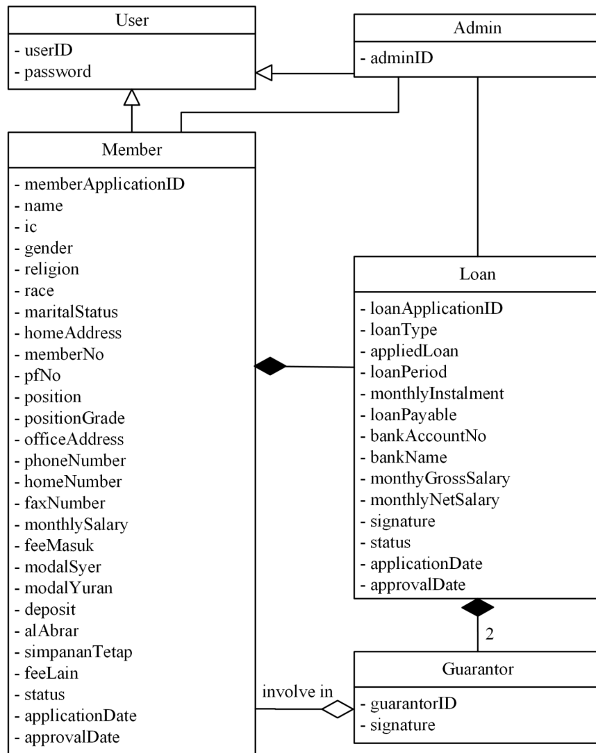
Figure 4.14 Class Diagram for Loan Module
