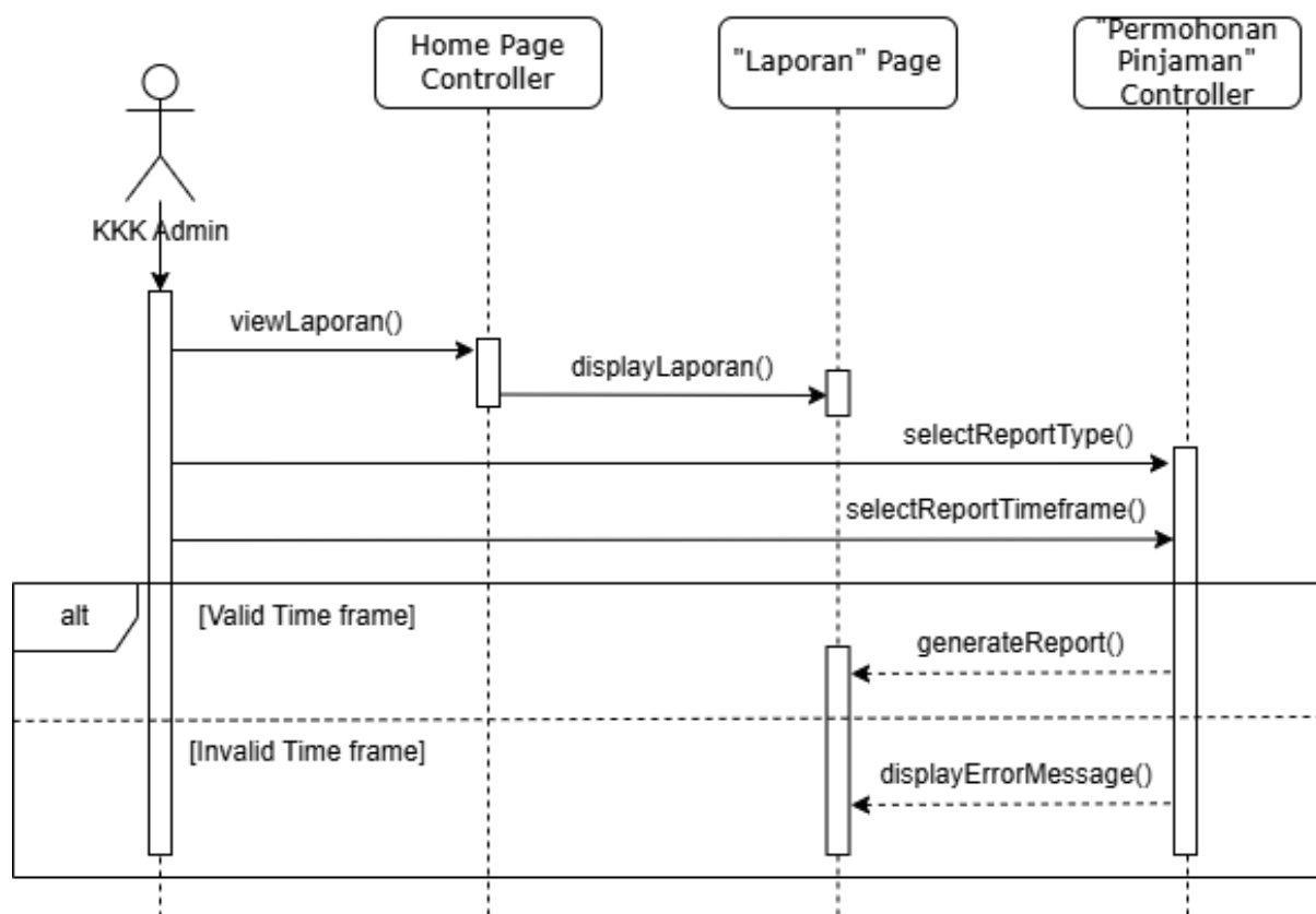
Figure 2.23: Sequence Diagram for Generate Report
