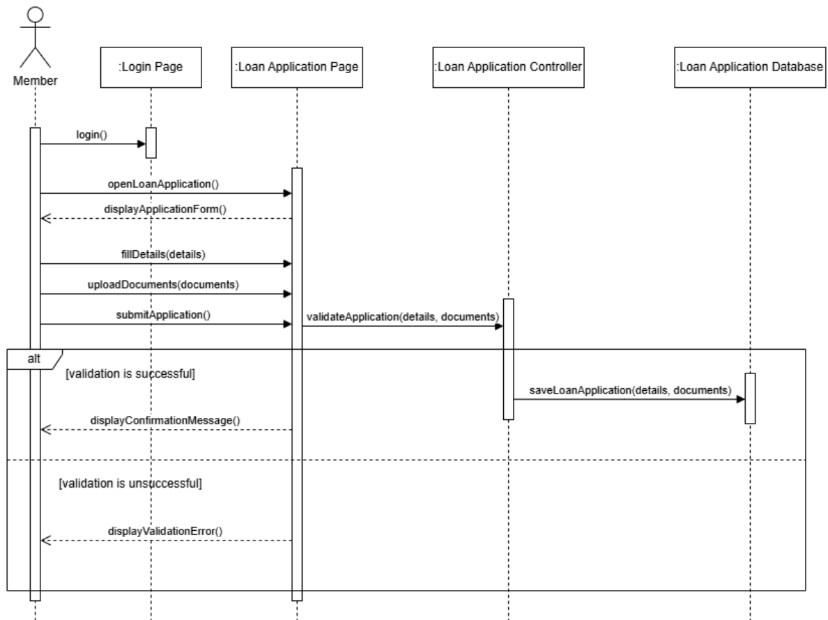
Figure 2.13: Sequence Diagram for Apply for a Loan
