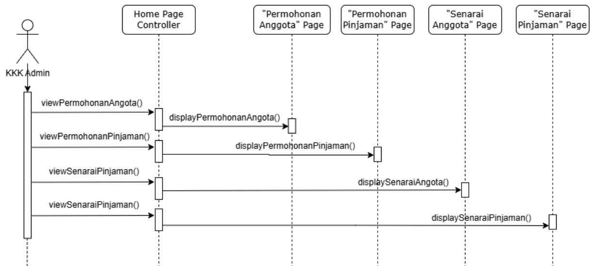
Figure 4.24: SD007 Sequence Diagram for View List
