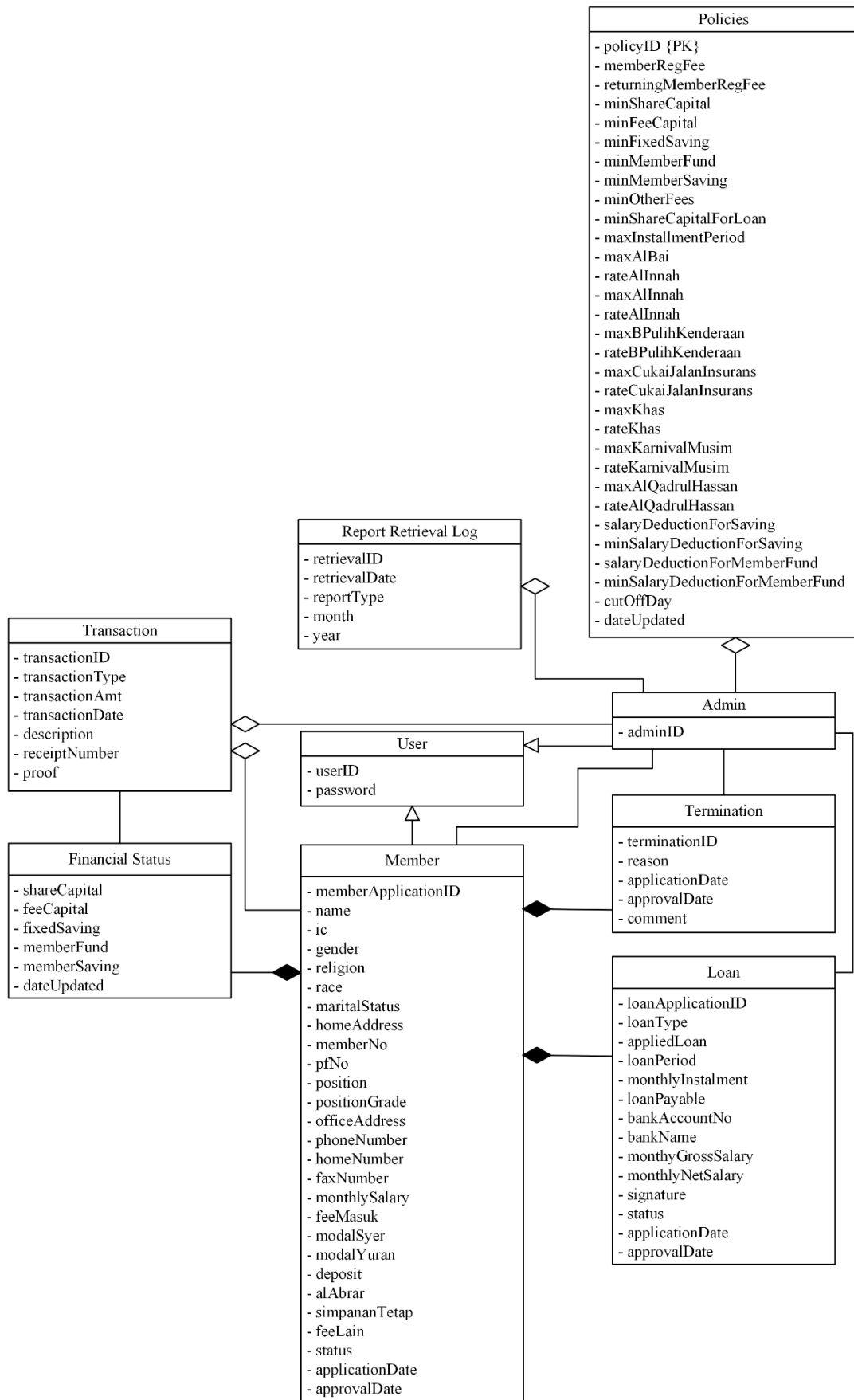
Figure 4.17 Class Diagram for Admin Reporting Module
