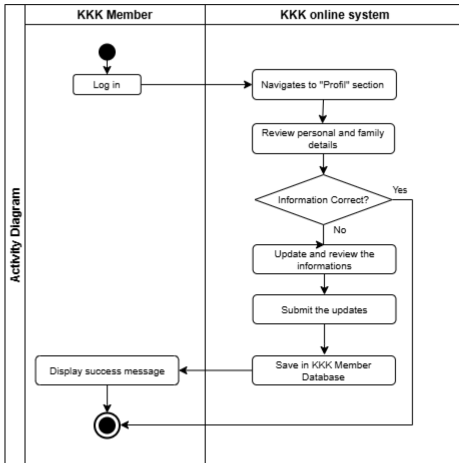
Figure 2.8: Activity Diagram for Update User Profile
