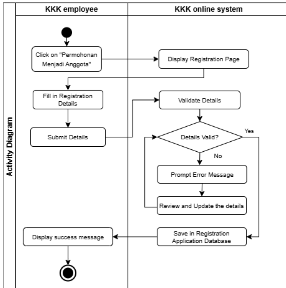
Figure 2.6: Activity Diagram for Apply Membership
