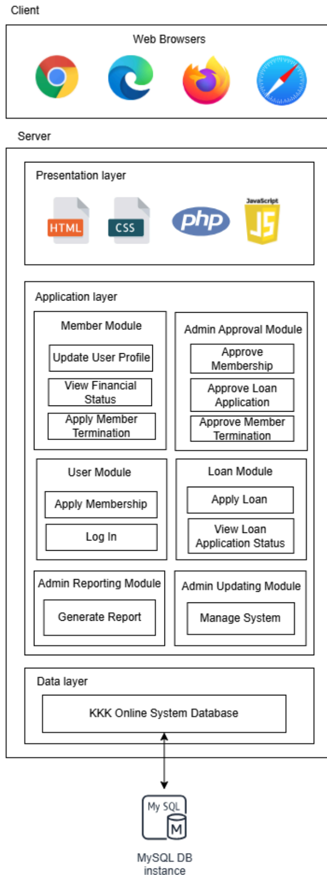
Figure 4.3 Architecture Diagram for KKK Online System
