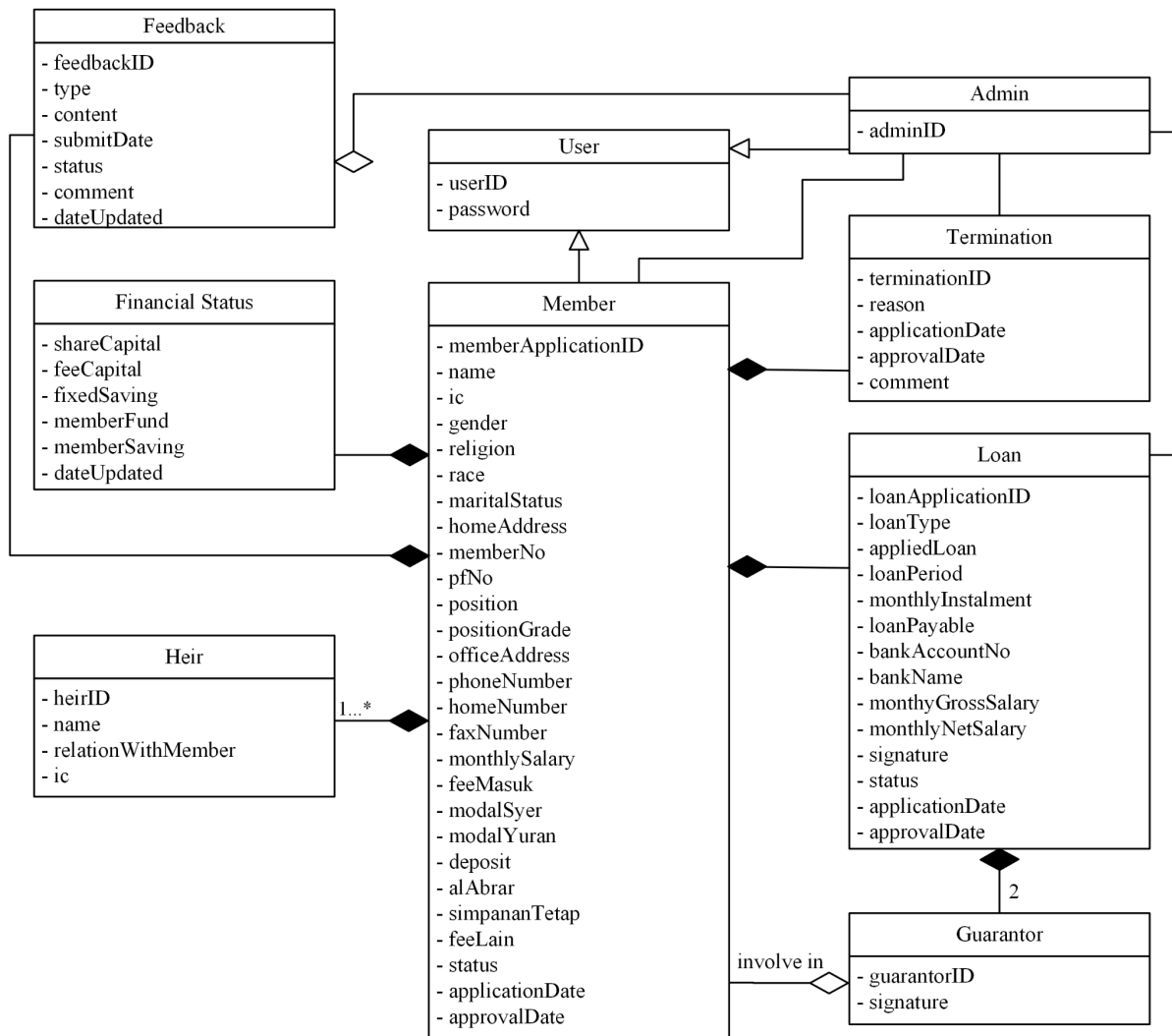
Figure 4.15 Class Diagram for Admin Approval Module
