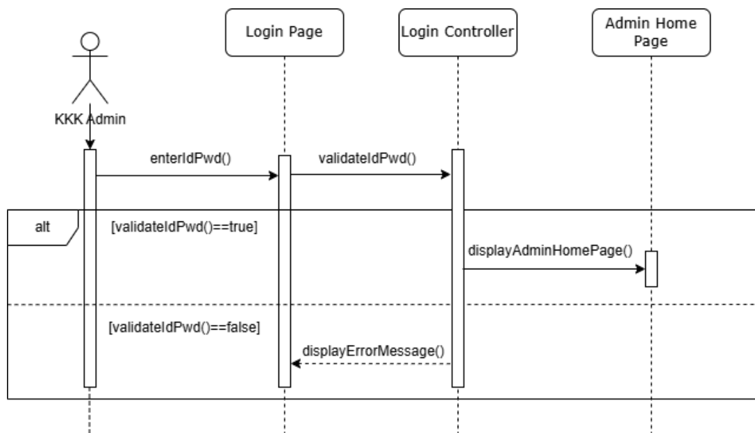
Figure 2.9: Sequence Diagram for Login
