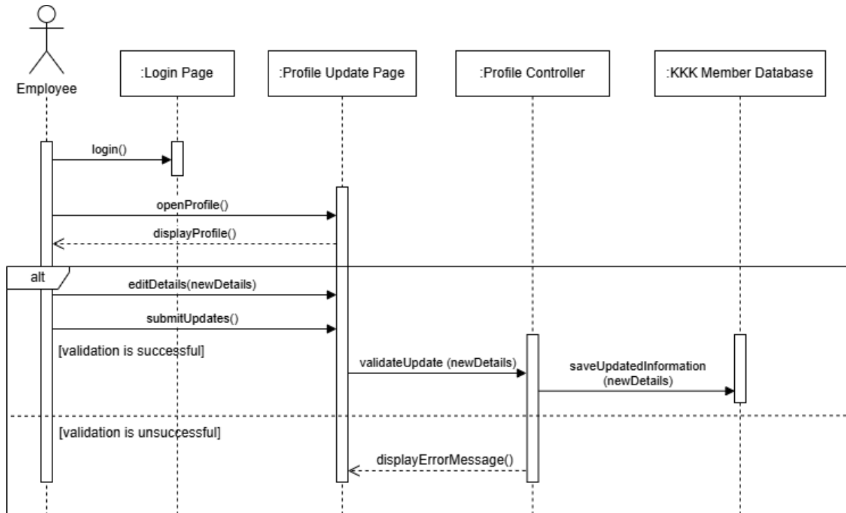
Figure 4.20: SD003 Sequence Diagram for Update User Profile
