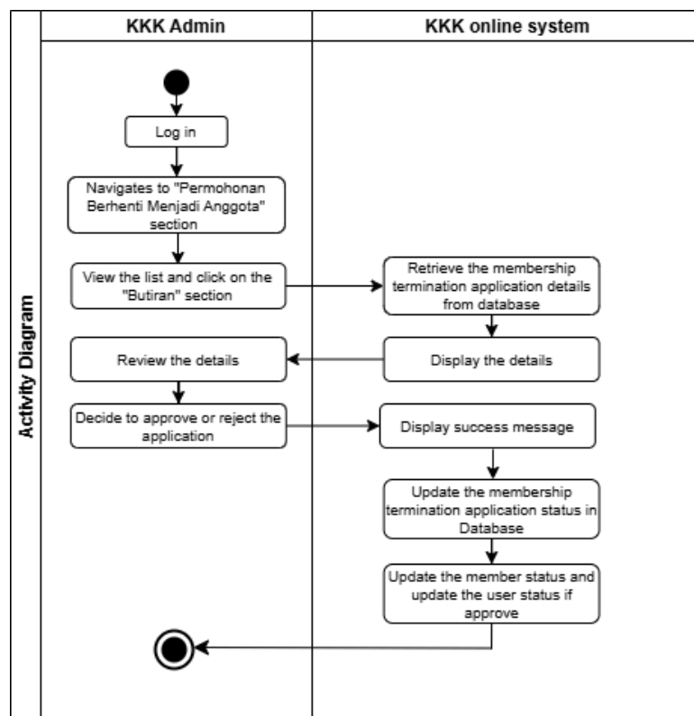
Figure 2.28: Activity Diagram for Approve Membership Termination
